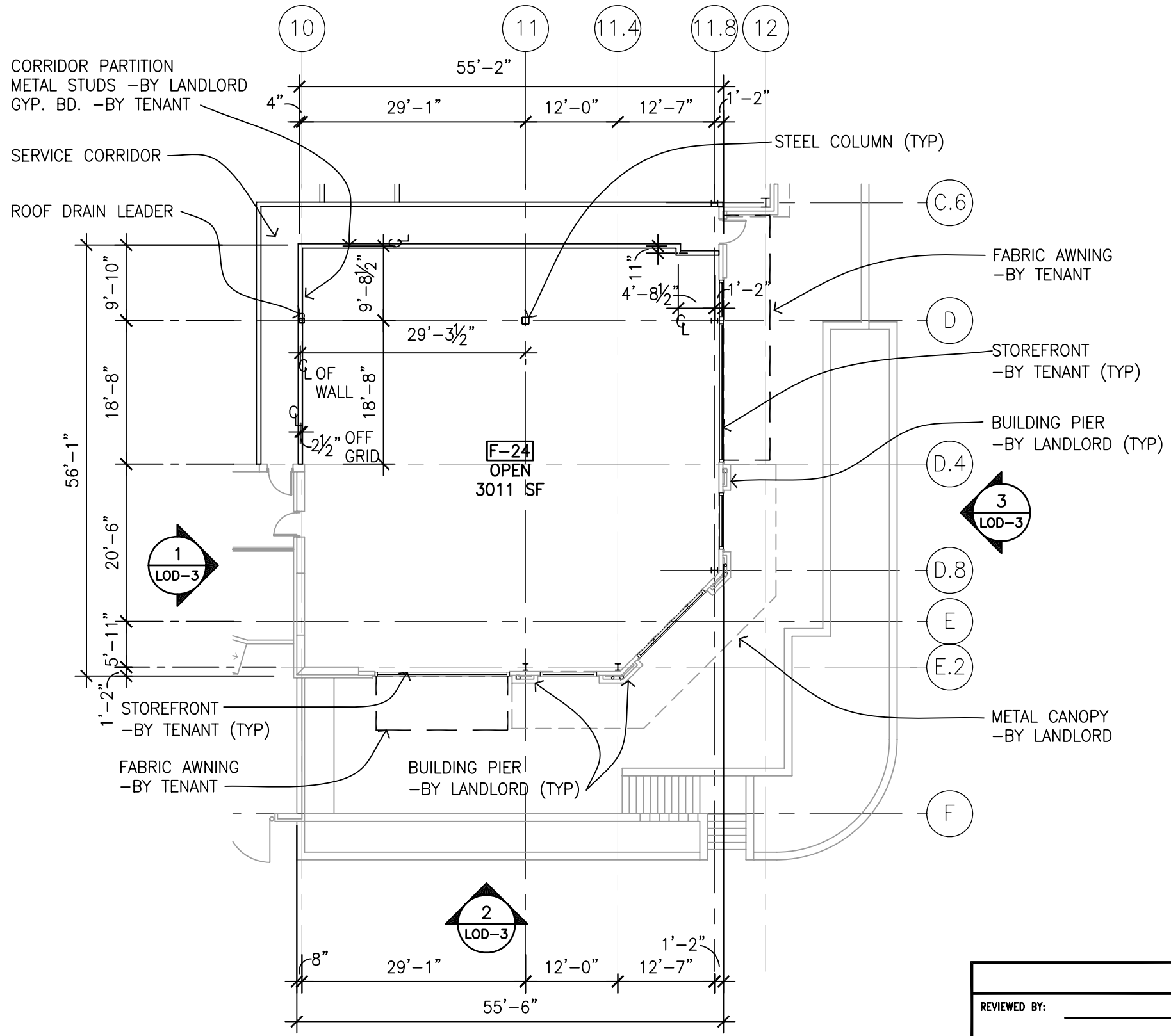
1 SPACE PLAN 1/16" = 1'-0"
